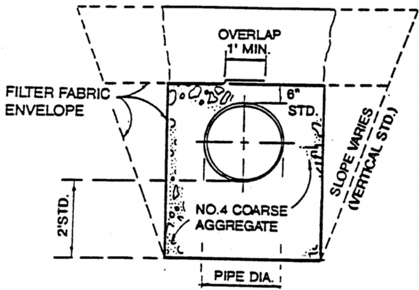
STANDARD CROSS SECTION NTS
