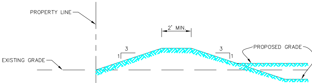
BERM DETAIL NTS
