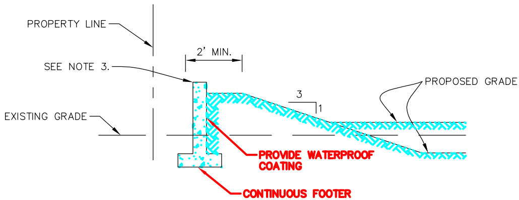
ALTERNATE RETAINING WALL DETAIL NTS
